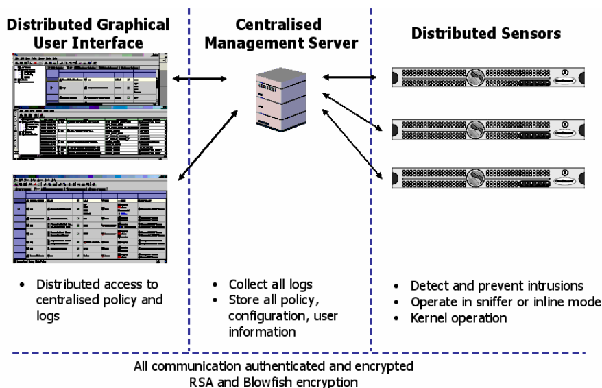
Figure 1 - NetScreen-IDP: Architecture
