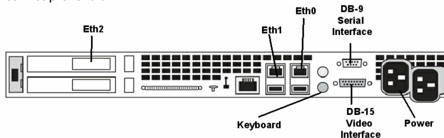
Figure 2 - NetScreen-IDP: Sensor rear panel
